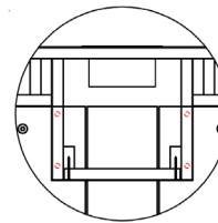
Horizontal Wire Management Trough (included with wire management up charge)
